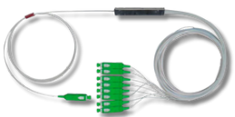
Mini Splitter PLC SP (APC) x SC (APC) NX-NMPL1XX110110441 Bitola de 2,00mm Tamanho de 3,00mts
